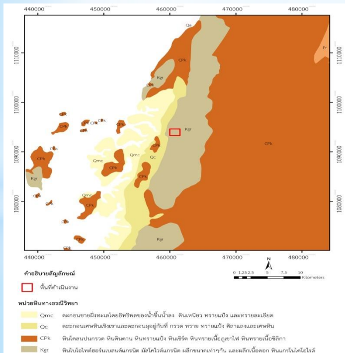
Fig. 2 : Geological map of Ranong Provinc
