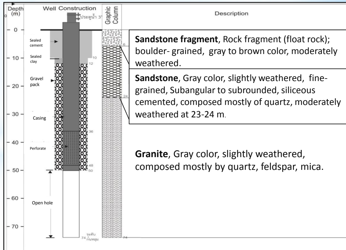
Fig.4 : Hot spring well construction and lithological logging
