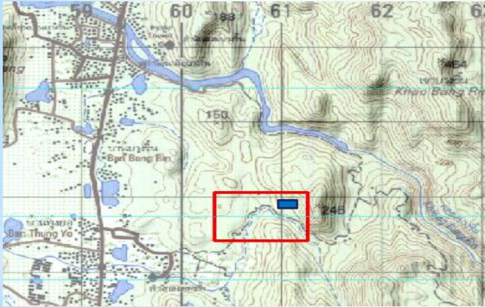
Fig. 1 Topographic map of Bangrin subdistrict.
