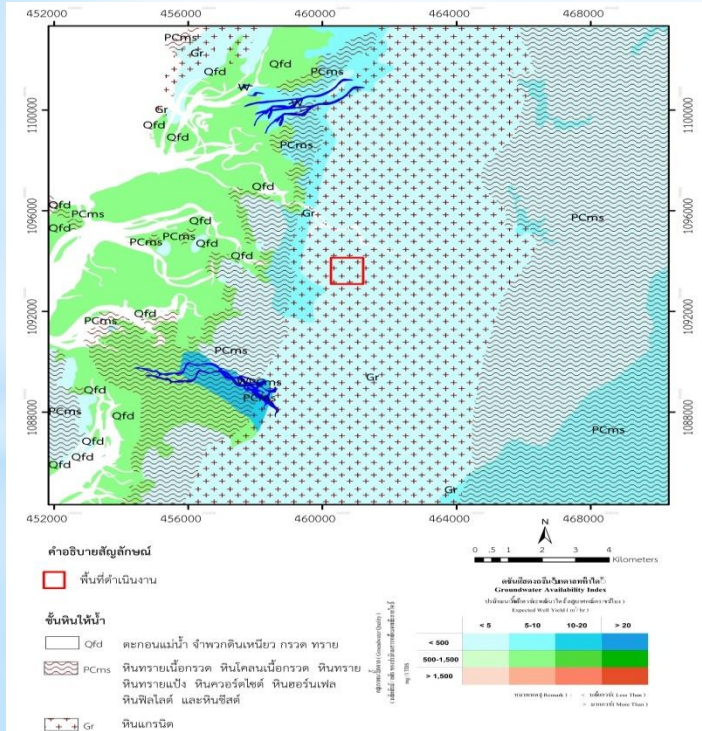
Fig. 3: Groundwater map of Ranong Provinc
